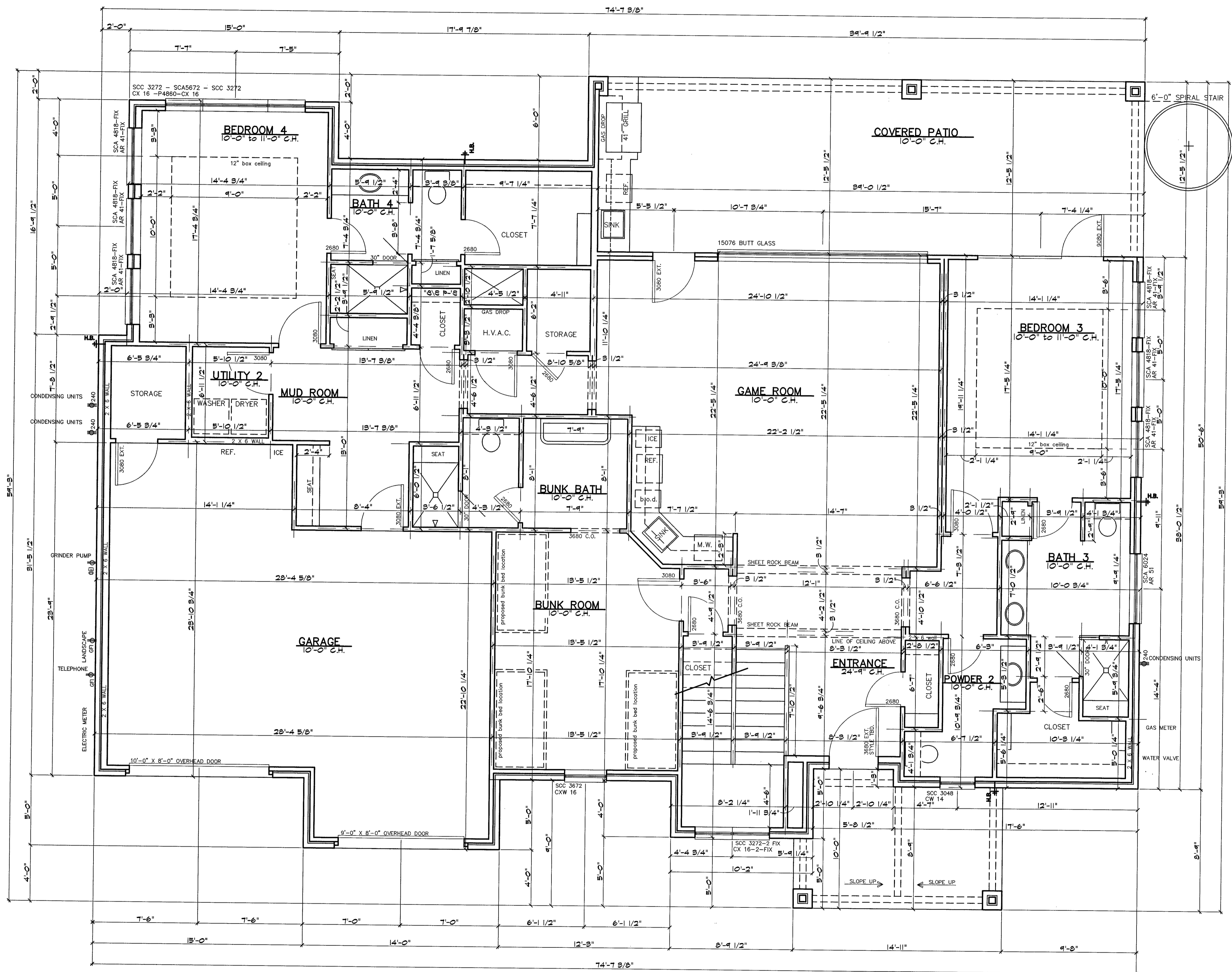
1 GROUND LEVEL FLOOR PLAN SCALE: 1/4"=1'-0"
